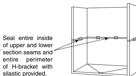
Fig. 3 – Bin Cutaway
