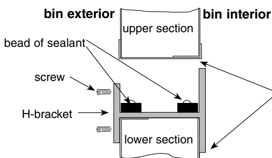
Fig. 2 – Cross Section, Side View
